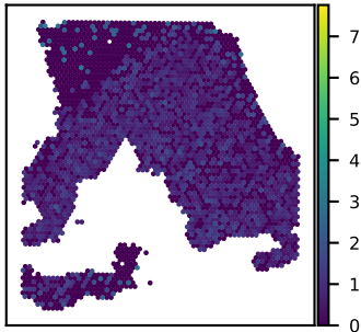
SNU18A PPP2R2A expression Moran's I = 0.07
