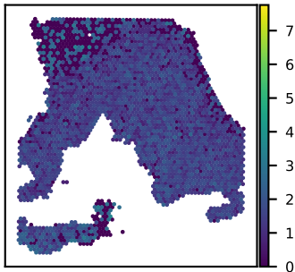
SNU18A UBE2V1 expression Moran's I = 0.13
