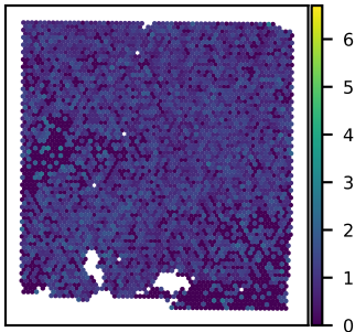
SNU43A TRIM56 expression Moran's I = 0.06
