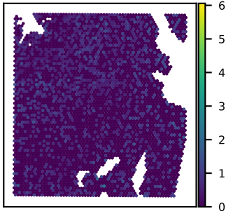
SNU51A SH3BGR expression Moran's I = 0.01
