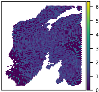
SNU24A C9orf78 expression Moran's I = 0.10
