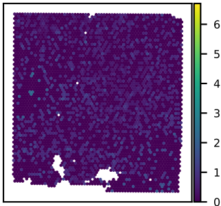
SNU43A C12orf45 expression Moran's I = 0.01
