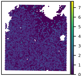
SNU21B MPHOSPH8 expression Moran's I = 0.09
