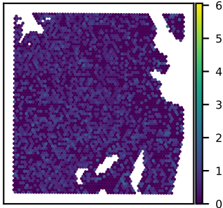
SNU51A CHAMP1 expression Moran's I = 0.01
