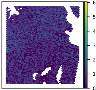
SNU51A CCND3 expression Moran's I = 0.08
