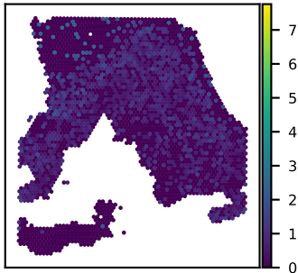
SNU18A ADAMTSL4 expression Moran's I = 0.12
