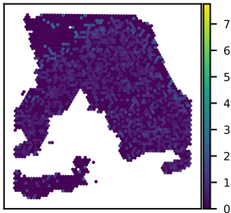
SNU18A GTPBP3 expression Moran's I = 0.06
