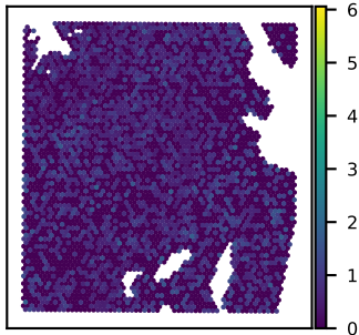
SNU51A FOXO1 expression Moran's I = 0.02
