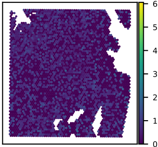
SNU51A COMMD5 expression Moran's I = 0.01
