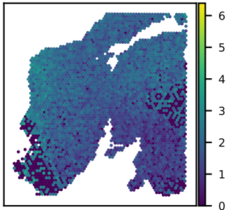
SNU24A ALDOC expression Moran's I = 0.30
