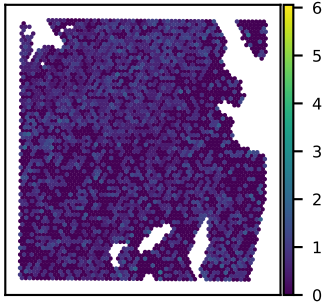
SNU51A RHOG expression Moran's I = 0.04
