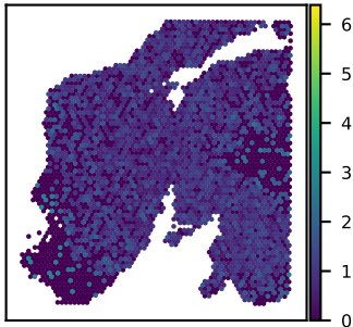
SNU24A SARM1 expression Moran's I = 0.06
