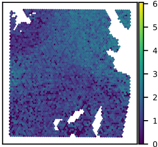
SNU51A MTURN expression Moran's I = 0.38
