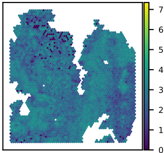
SNU27B SERPINA3 expression Moran's I = 0.40
