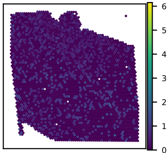
SNU27A BGLAP expression Moran's I = 0.02
