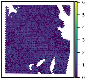
SNU51A NDUFV3 expression Moran's I = 0.02
