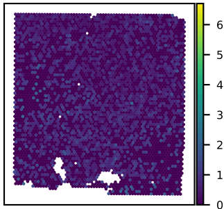
SNU43A TMEM161A expression Moran's I = 0.02
