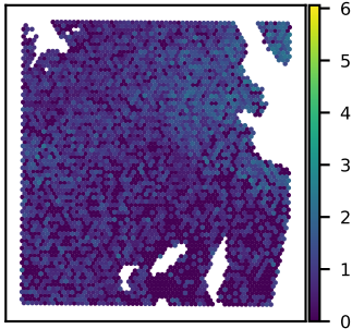
SNU51A PPP3CA expression Moran's I = 0.23
