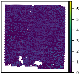
SNU43A CAMTA2 expression Moran's I = 0.01
