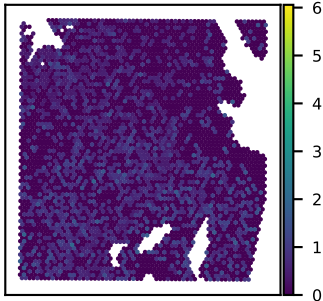
SNU51A PALM3 expression Moran's I = 0.05
