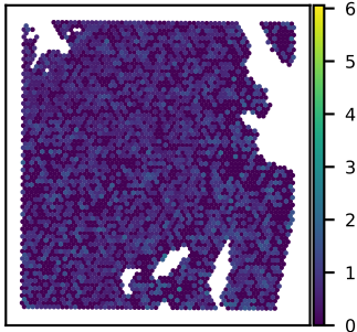
SNU51A MRNIP expression Moran's I = 0.02
