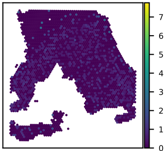
SNU18A NEURL2 expression Moran's I = 0.03
