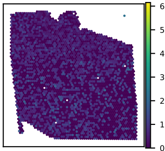
SNU27A C11orf71 expression Moran's I = 0.02
