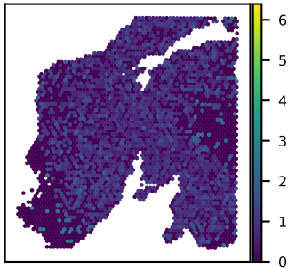
SNU24A PPFIBP1 expression Moran's I = 0.08
