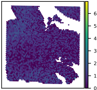
SNU24B TMEM14A expression Moran's I = 0.15
