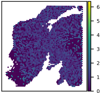
SNU24A MPHOSPH8 expression Moran's I = 0.09
