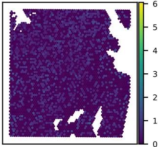
SNU51A FAIM expression Moran's I = 0.01
