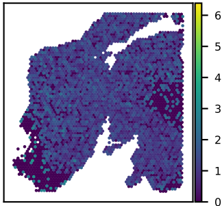
SNU24A TMEM184B expression Moran's I = 0.10
