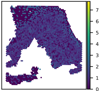
SNU18A SEMA5A expression Moran's I = 0.11
