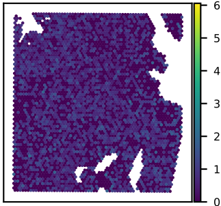
SNU51A NUP85 expression Moran's I = 0.03
