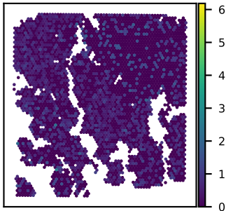
SNU16B CSNK1G3 expression Moran's I = 0.03
