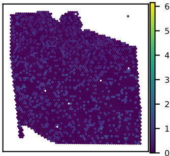
SNU27A SLC35B4 expression Moran's I = 0.02
