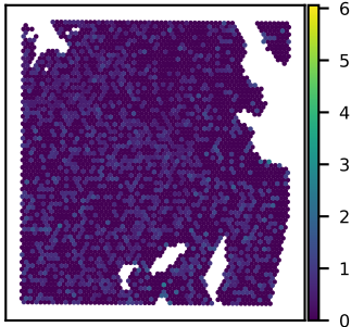
SNU51A DHX34 expression Moran's I = 0.01
