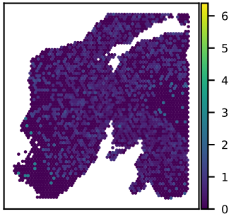
SNU24A ZNF274 expression Moran's I = 0.03
