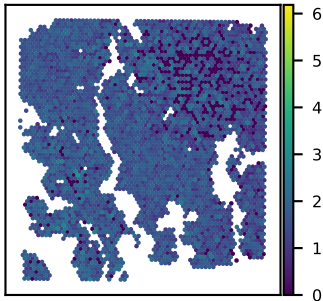
SNU16B SNRNP200 expression Moran's I = 0.08
