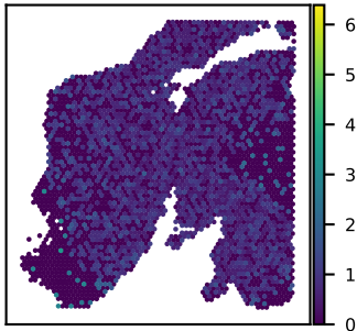
SNU24A TBC1D23 expression Moran's I = 0.05
