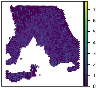
SNU18A LPGAT1 expression Moran's I = 0.08
