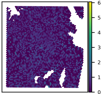
SNU51A SNAPIN expression Moran's I = 0.02
