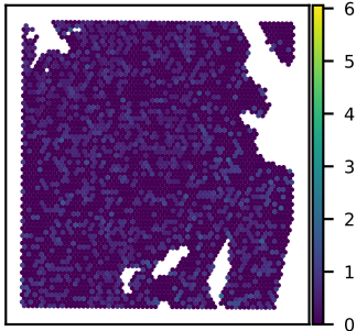
SNU51A STK36 expression Moran's I = 0.02
