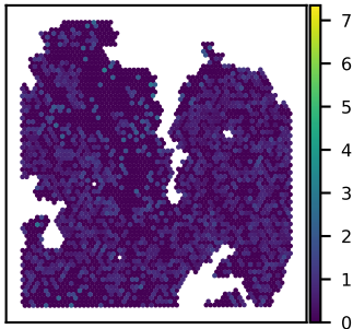
SNU27B C1orf216 expression Moran's I = 0.03
