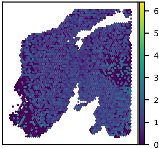
SNU24A LEPROTL1 expression Moran's I = 0.08
