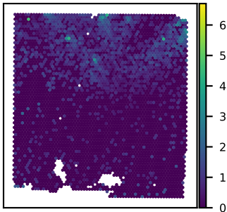
SNU43A IGHG2 expression Moran's I = 0.45
