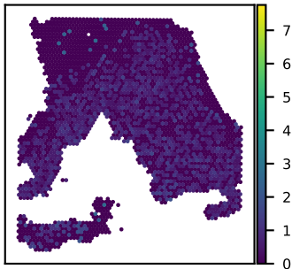
SNU18A ZC3H7B expression Moran's I = 0.10
