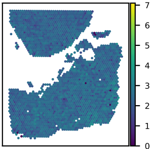
SNU25A SNRNP70 expression Moran's I = 0.12
