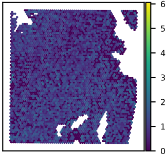
SNU51A NDUFA7 expression Moran's I = 0.05
