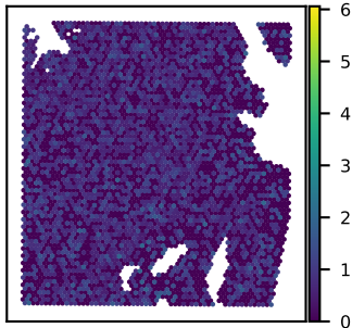
SNU51A MGAT5 expression Moran's I = 0.01
